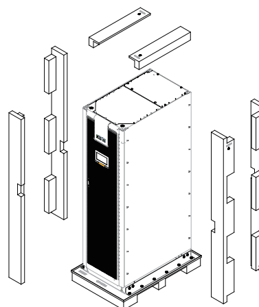
图4-3: 移除缓冲材
